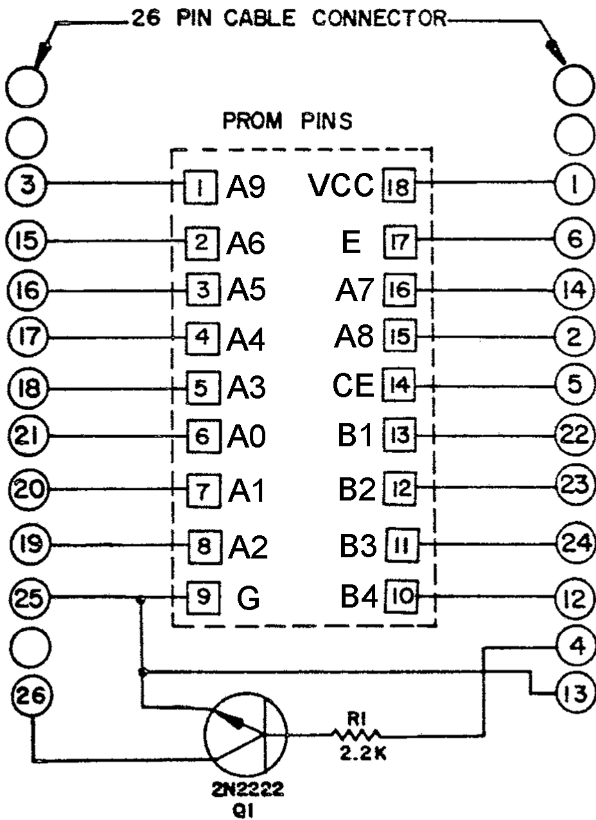
Fig. 2. SCHEMATIC DIAGRAM, ADAPTER 715-1036
